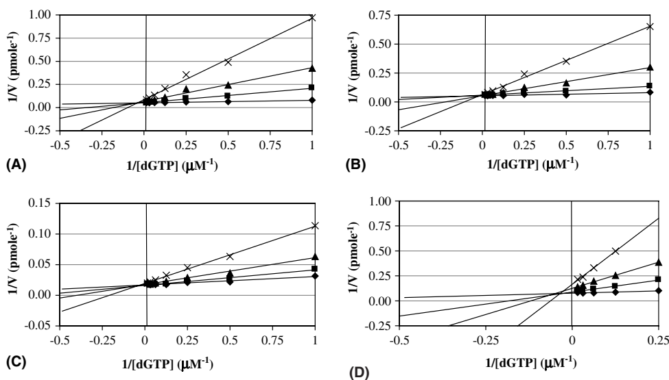
Figure 1. Double reciprocal (Lineweaver–Burk) plots demonstrating effect of varying dGTP concentration on inhibition of pol III species. 12 Panel A, B.s. pol III C + 3c. Panel B, B.s. pol III C + 4o. Panel C, B.s. pol III E + 4o. Panel D, E.c. pol III E + 4o. Inhibitor concentrations: (■) 3 \times K_i ; (▲) 10 \times K_i ; (×) 30 \times K_i ; (◆) no inhibitor.
